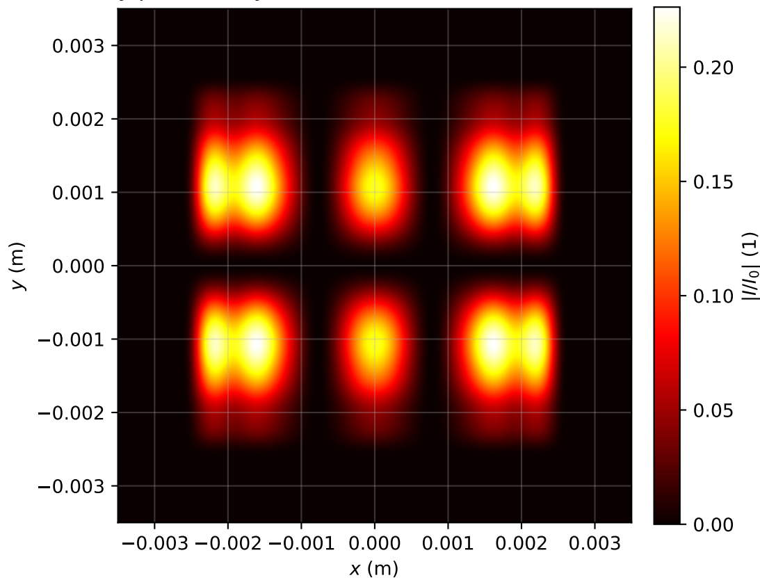
Intensity profile I(x, y, z = 3.901)/I_0 , P_{in}=0.5P_{cr} , artificial time
